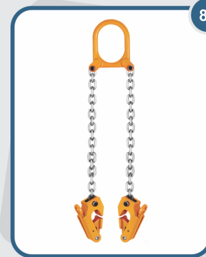
DRUM LIFTING CLAMP
