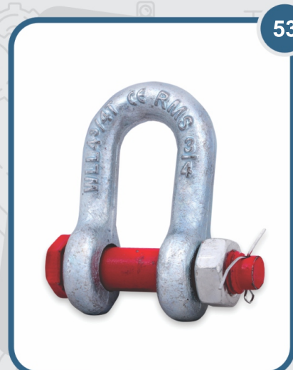
ALLOY STEEL G80 DEE SHACKLE NUT BOLT TYPE
